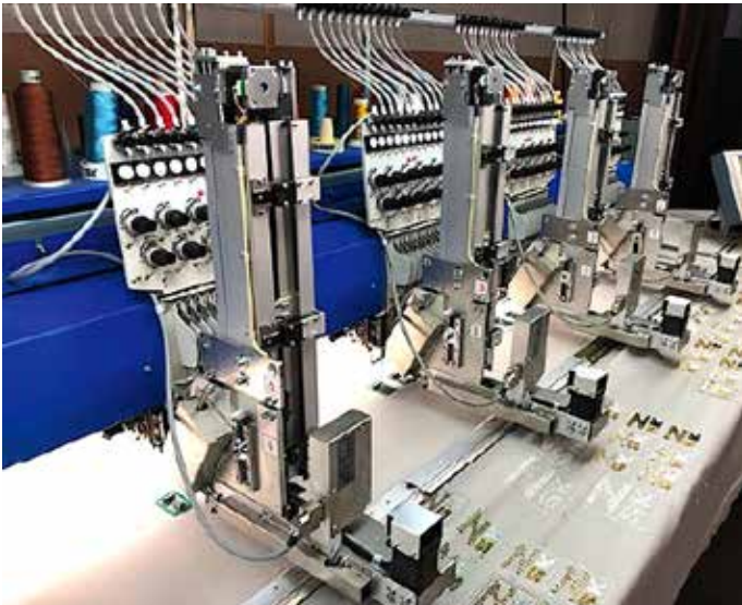
POB E30 PLACEMENT DEVICE
