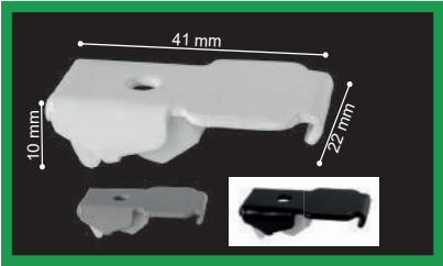
Soporte techo Ceiling Bracket / Support Plafond
