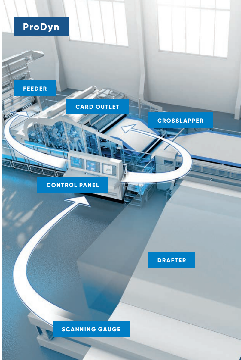
ProDyn system
