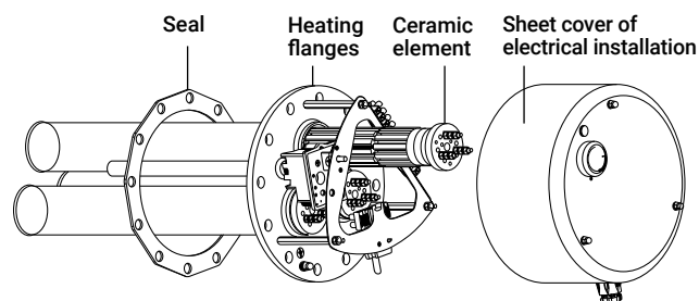
TPK – THREE-PHASE
